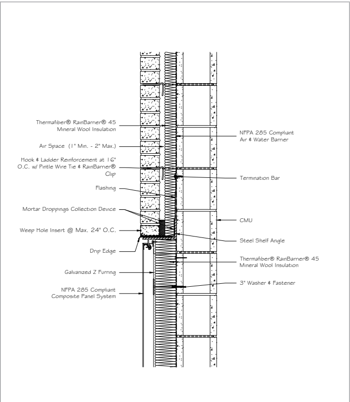
32 Transition Head, CMU
