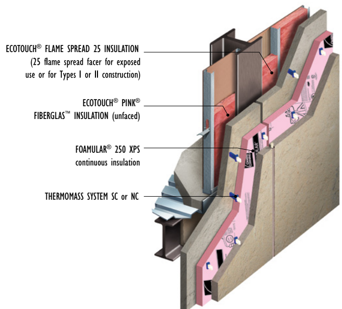
Insulated Precast
