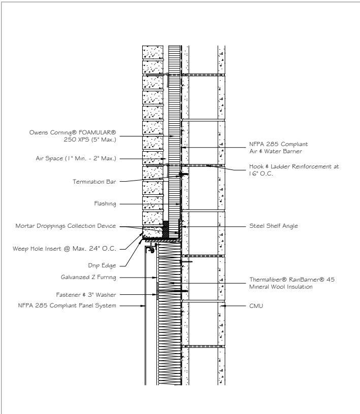
31 Transition Head, CMU
