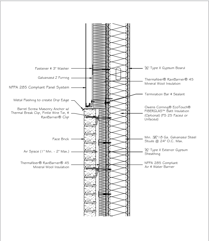
30 Transition Sill, Steel Stud
