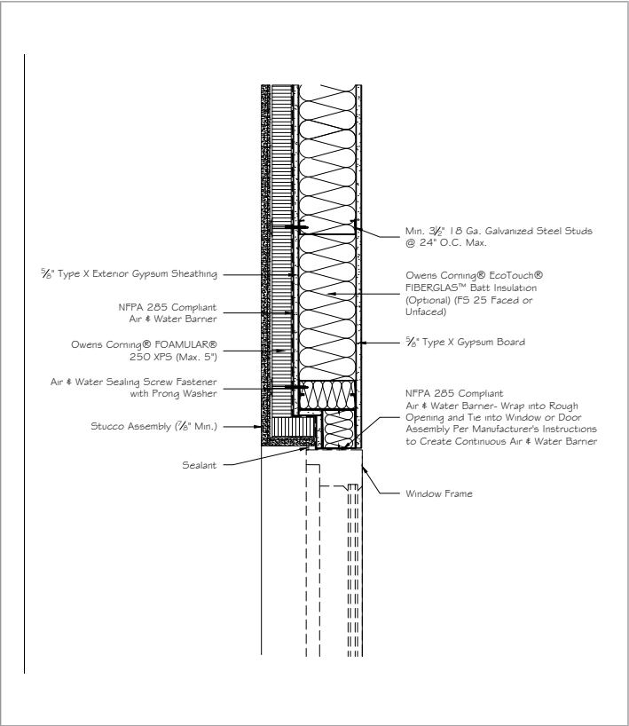
16 FOAMULAR® XPS, Stucco Jamb
