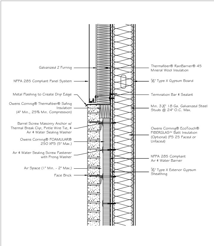
29 Transition Sill, Steel Stud
