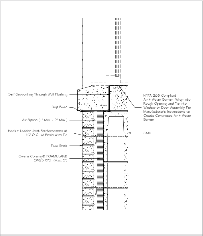
14 FOAMULAR® XPS, CMU Sill
