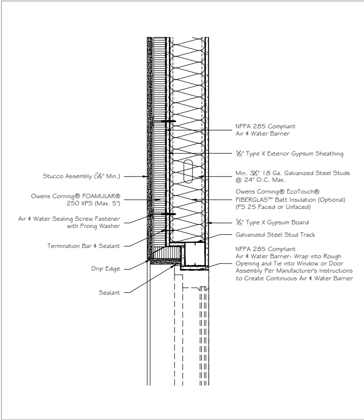
15 FOAMULAR® XPS, Stucco Head
