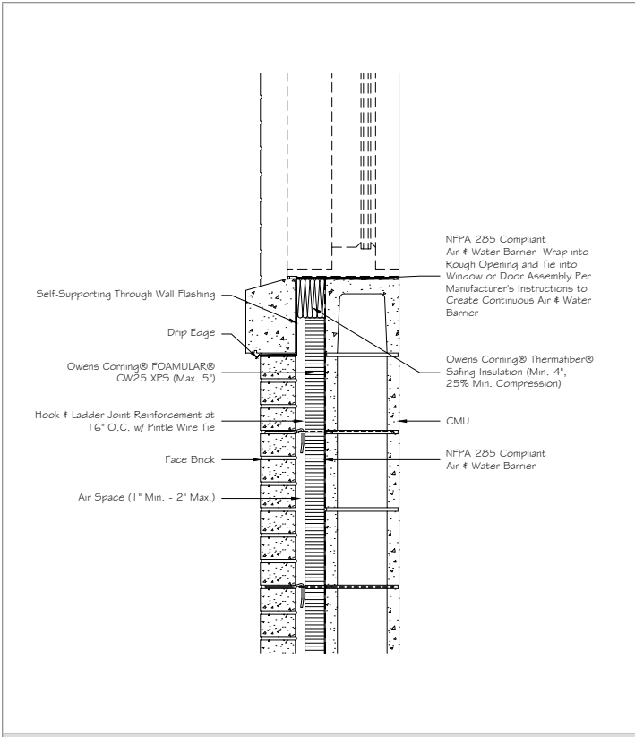
13 FOAMULAR® XPS, CMU Sill
