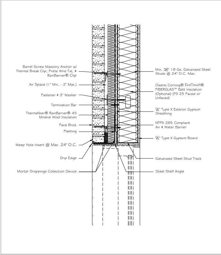
37 Thermafiber® MW, Steel Stud Head
