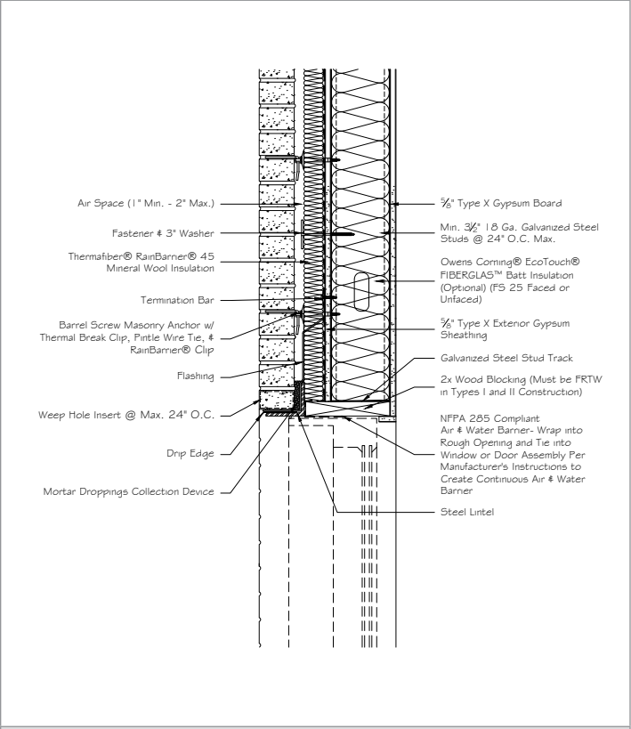
38 Thermafiber® MW, Steel Stud Head
