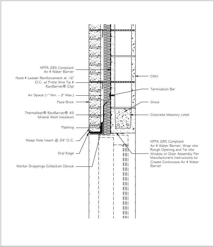
45 Thermafiber® MW, CMU Head
